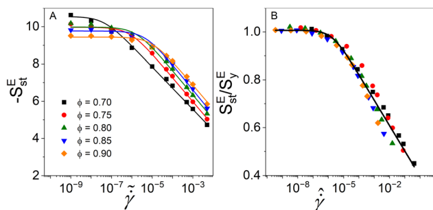
Fig. 7 Steady-state excess entropy, -S^E_{st} , as a function of shear rate, \dot{\gamma} , and (B) rescaled excess entropy S^E_{st}/S^E_{\dot{\gamma}} , where S^E_{\dot{\gamma}} is the excess entropy in the dynamic yield point, as a function of the rescaled shear rate, \hat{\gamma} . The solid line shows the logarithmic fit to the data.
