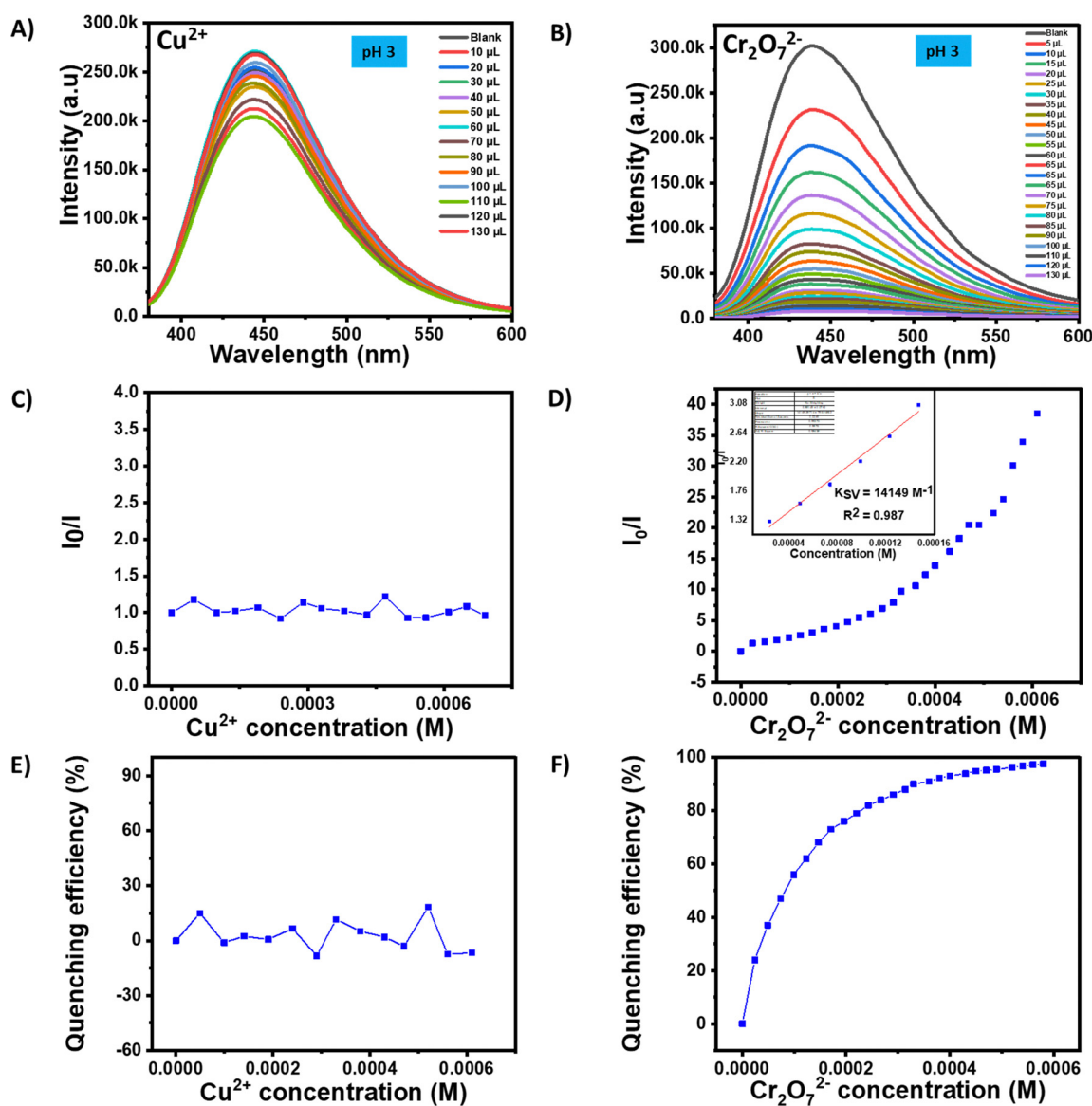
Fig. 6 (A) and (B) Fluorescence emission spectra of NANO-PAMAM-CHT in the presence of \text{Cu}^{2+} and \text{Cr}_2\text{O}_7^{2-} at pH 3. (C) and (D) K_{sv} plot of NANO-PAMAM-CHT with the addition of \text{Cu}^{2+} and \text{Cr}_2\text{O}_7^{2-} at pH 3. (E) and (F) Quenching efficiency plot of NANO-PAMAM-CHT with the addition of \text{Cu}^{2+} and \text{Cr}_2\text{O}_7^{2-} at pH 3.
