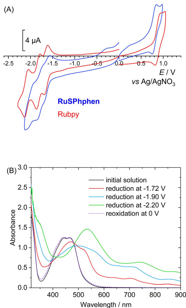
Fig. 1 (A) Cyclic voltammograms in DMF, 0.1 M [Bu 4 N]ClO 4 at a glassy carbon electrode ( \varnothing = 3 mm, \nu = 100 mV s -1 ) of solutions of RuSPphen (0.44 mM, blue line) and Rubpy (0.3 mM, red line). (B) UV-visible absorption spectral changes of the solution of RuSPphen (0.44 mM) in DMF, 0.1 M [Bu 4 N]ClO 4 , after three successive exhaustive reductions at (a) E = -1.72 V (formation of RuSPphen 5- also denoted as RuSPphen - ), (b) -1.90 V (formation of RuSPphen 6- ), and (c) -2.20 V (formation of RuSPphen 7- ) and (d) after a reoxidation at 0.0 V (reformation of RuSPphen ). The optical path is 1 mm.
