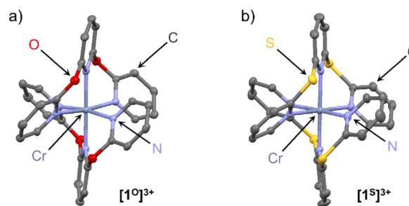
Fig. 1 Molecular structures of the trications of the chromium complexes (a) [ \mathbf{1}^{\text{O}} ][OTf] 3 and (b) [ \mathbf{1}^{\text{S}} ][OTf] 3 determined by XRD. Hydrogen atoms, counter ions and co-crystallised solvent molecules omitted. Thermal ellipsoids at 50% probability level.
