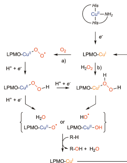
Scheme 3 Putative mechanisms to explain LPMO catalyzed hydroxylation: (a) the monooxygenase pathway and (b) peroxygenase pathway.
