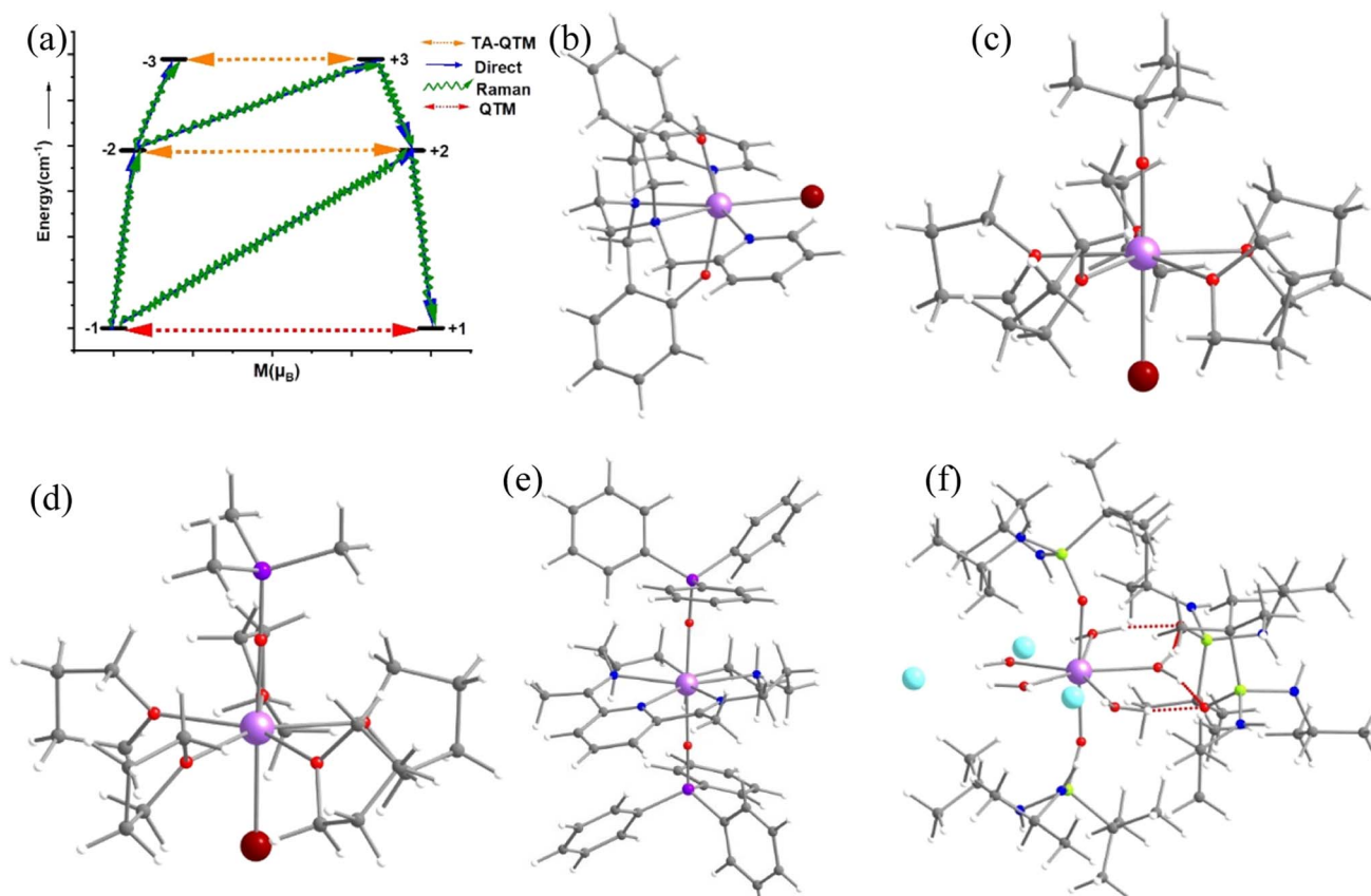
Fig. 1 (a) The general magnetisation relaxation diagram. Here, red arrows denote the QTM for the ground state and TA-QTM (orange) for the excited state. The blue arrows signify the direct/Orbach process. The green arrow implies the Raman process. The crystal structure of complexes (b) [Dy(bbpen)Br] 1, (c) [Dy(OCMe 3 )Br(THF) 5 ][BPh 4 ] 2, (d) [Dy(OSiMe 3 )Br(THF) 5 ][BPh 4 ] 3, (e) [Dy(L N5 )(Ph 3 SiO) 2 ](BPh 4 )·CH 2 Cl 2 4 and (f) [L 2 Dy(H 2 O) 5 ][I] 3 ·L 2 ·H 2 O 5. The hydrogens are omitted for clarity. Colour code: Dy-violet, I-cyan Br-brown, O-red, Si-purple, N-blue, and C-grey.
