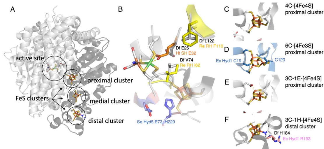
Fig. 4 The NiFe hydrogenase dimer. (A) Overview of the structure of prototypical hydrogenases, the large subunit (light grey) embeds the active site, and the small subunit (dark grey) a chain of FeS clusters. (B) The environment of the active site, showing the V74/L122/E25 (Sf Hyn numbering) residues in prototypical hydrogenases, 37,38 the residue E32 binding the Ni in the oxidised form of Ht SH, 39 the I62/F110 residues in Cupriavidus necator (Cn), previously known as Ralstonia eutropha MBH 40,41 (based on an AlphaFold model), and the E73 and H229 residues in S. enterica (Se) Hyd 5. 42 (C) The proximal [4Fe4S] cluster in prototypical NiFe hydrogenases. (D) The proximal [4Fe3S] cluster in group 1d hydrogenases, coordinated by two supernumerary cysteines, C19 and C120 ( E. coli Hyd 1 numbering). 43–45 (E) The proximal cluster coordinated by 3 cysteines and one aspartate in the AH enzyme from C. necator . 46 (F) The histidine ligated distal cluster in prototypical NiFe hydrogenases, 47 and the arginine residue substituted in E. coli Hyd 1. 48
