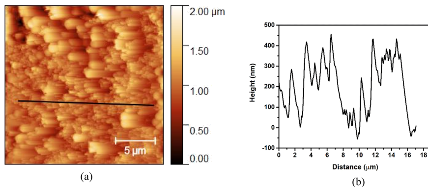
Fig. 4 AFM image of the \text{TiO}_2 film deposited on a glass surface: (a) surface analysis, and (b) height profiling.
