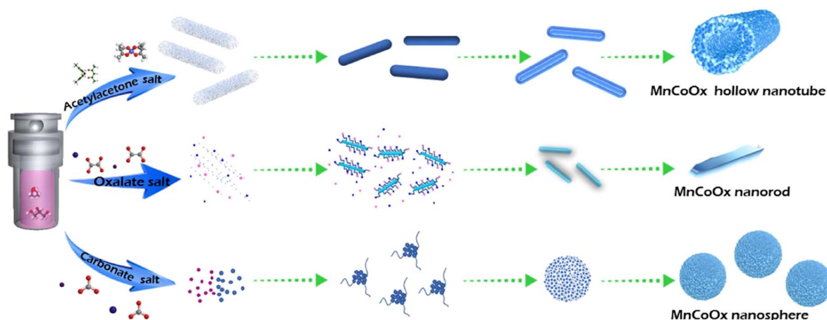
Fig. 5 The schematic illustration of the formation of the hollow nanotube, nanorod, and nanosphere of \text{MnCoO}_x oxides (eeprented from ref. 53. Copyright 2021, with permission from Elsevier).
