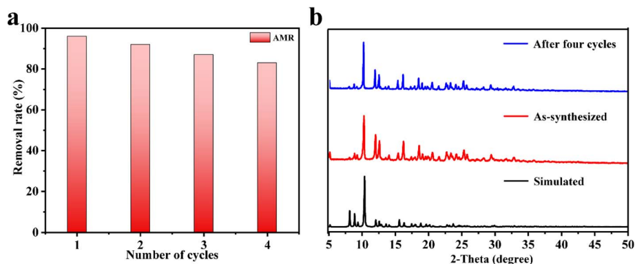
Fig. 5 (a) The recyclability tests of 1 towards the adsorption of aqueous AMR (20 mg L -1 ) in water and (b) PXRD patterns of 1 as-synthesized and after four cycles.
