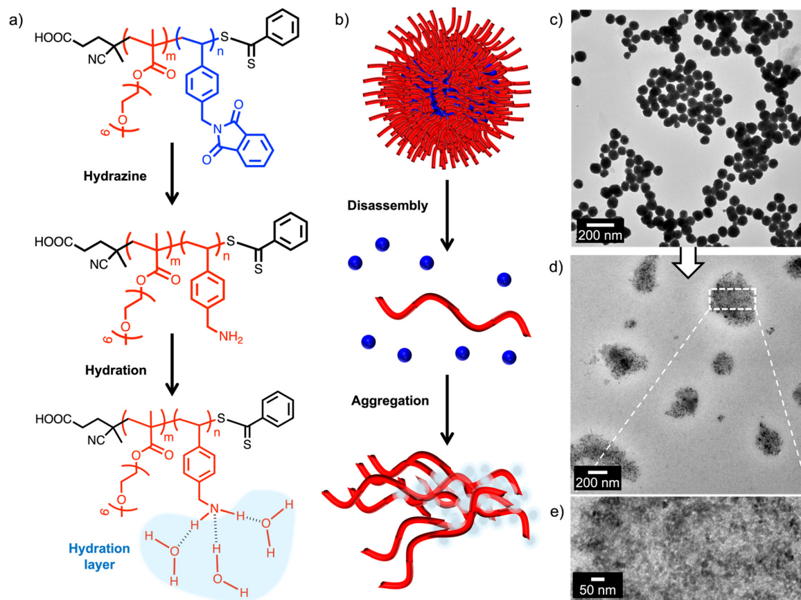
Fig. 6 Schematic representation for disassembly of PEGMA 15 - b -VBzPHT n to PEGMA 15 - b -(VBzNH 2 ) n . (a) Chemical structure, (b) schematic disassembly and aggregation process, (c) representative TEM images for P2 before hydrazine treatment, (d & e) P2 after deprotection and aggregation after hydrazine treatment for 20 h.
