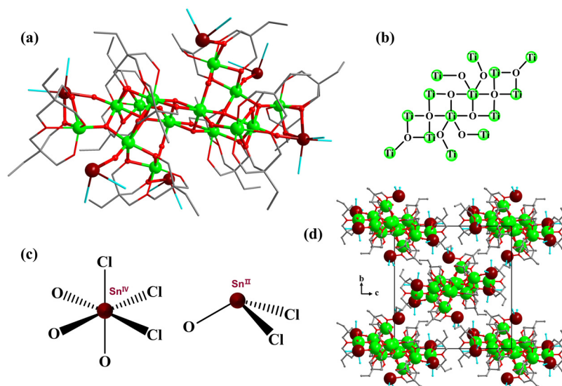
Fig. 4 (a) The cluster structure of TOC-57. (b) Connection diagram of Ti atoms through bridging an O atom in TOC-57. (c) Coordination spheres of the Sn atoms in TOC-57. (d) The packing mode of TOC-57.
