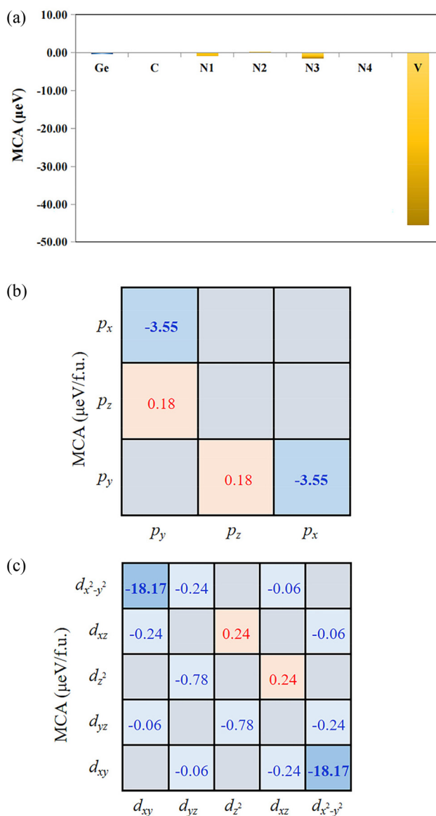
Fig. 8 (a) Atom-resolved MCA energy and orbital-resolved MCA energies of (b) V-p and (c) V-d for VCGeN 4 .
