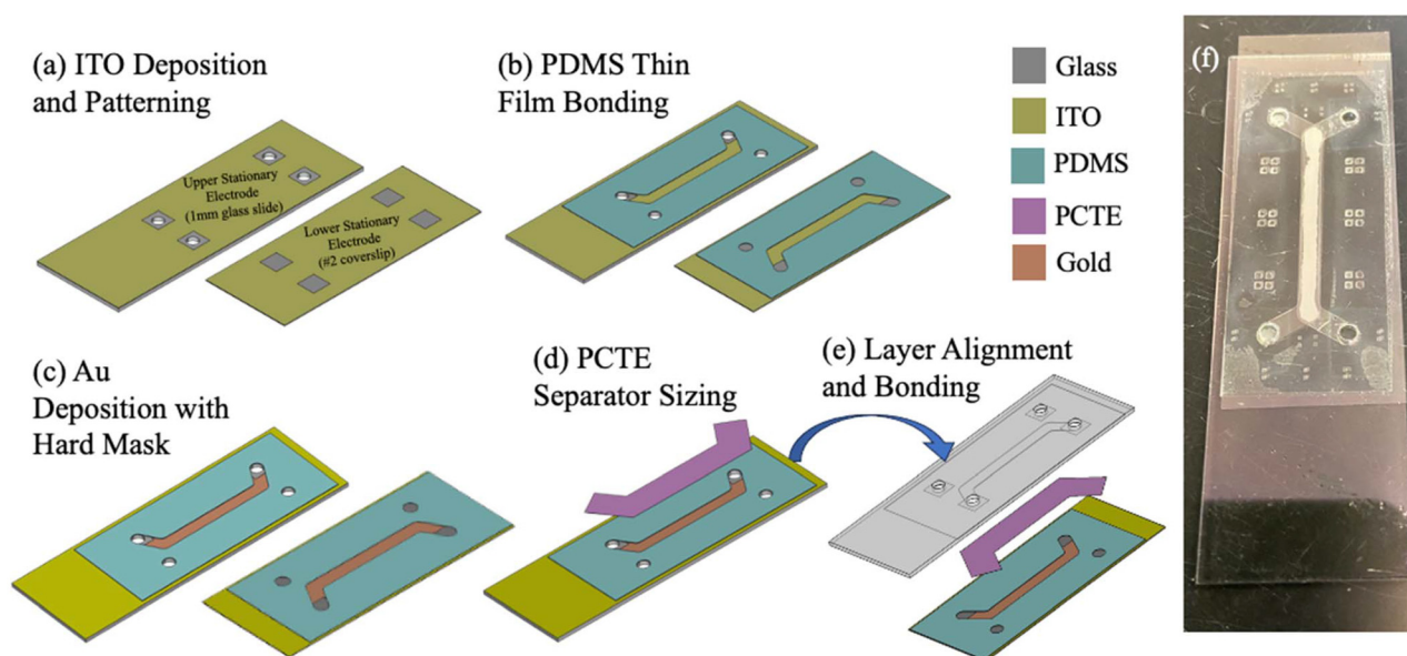
Fig. 2 (a) Visualization of the stationary electrodes after ITO has been sputtered and etched. (b) The PDMS channels bonded to the stationary electrodes. (c) The deposition of gold into the charging area. (d) Separator alignment after it has been cut to size. (e) The final step where the layers are aligned and epoxied together. (f) An image of a completed \mu -EFC.
