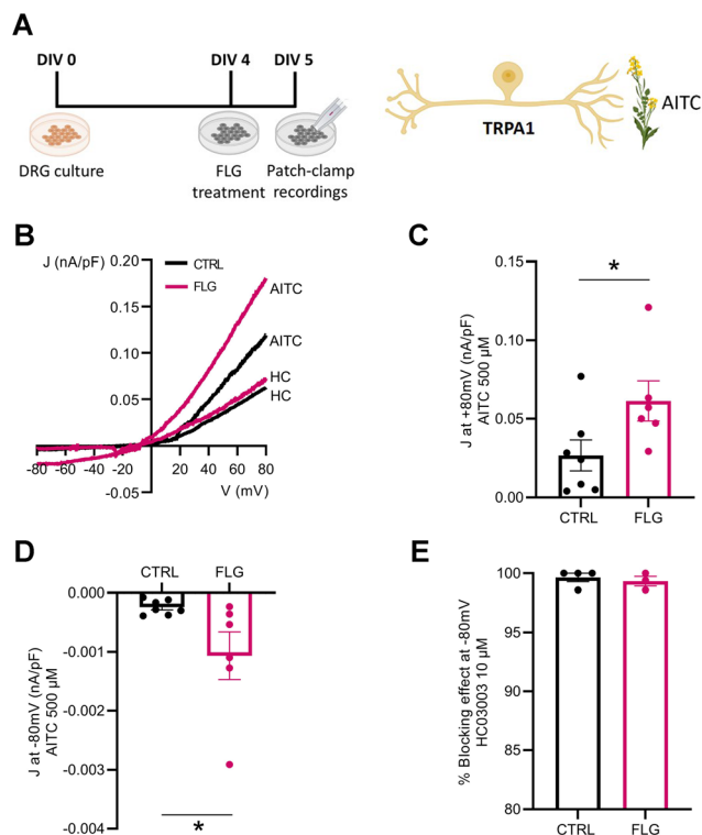
Fig. 7 (A) Timeline of the experiments (left) and cartoon of the TRPA1-specific agonist allyl isothiocyanate (AITC, 500 \mu M) used for the electrophysiological recordings (right). (B) Current density/voltage ( J/V ) relationships of TRPA1 channel activated by AITC in control untreated (CTRL) and FLG-treated (10 \mu g mL -1 ) DRG neurons. (C) and (D) Quantitative evaluation of whole-cell currents recorded at +80 mV and -80 mV in CTRL and FLG-treated neurons (CTRL, n = 7 ; FLG, n = 6 ). (E) Quantitative evaluation of the net percent effect of HC03003 (10 \mu M) blockade on AITC evoked currents under both conditions studied (CTRL, n = 4 ; FLG, n = 3 ). Data are expressed as means \pm SEM. Unpaired Student's t -test; * p < 0.05 .
