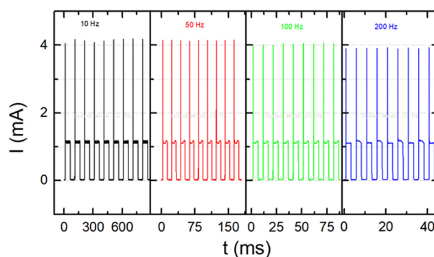
Fig. 9 I - t curves for the Ag@40 device at different chopper frequencies and at a fixed power density of 317 \text{ mW cm}^{-2} .
