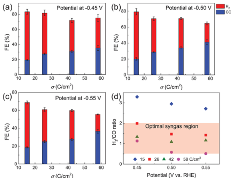
Fig. 30 The FEs of \text{H}_2 and CO production on OD-Cu NPs were measured at different applied potentials: (a) -0.45\text{ V} , (b) -0.50\text{ V} , and (c) -0.55\text{ V} . The controllable composition of syngas varies depending on the applied potentials (d). Reproduced with permission from ref. 331. Copyright 2020, American Chemical Society.
