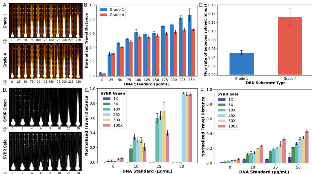
Fig. 2 Optimization of distance-based detection of dsDNA. A. Representative fluorescent images of dsDNA standards (0 to 250 \mu\text{g mL}^{-1} ) in grade 1 (top) and grade 4 (bottom) Whatman TM paper DBD substrates using 100 \times SYBR ® Safe intercalating dye. B. Graph of normalized travel distance as a function of concentration of dsDNA in grade 1 (blue) and 4 (red) substrates. C. Graph of flow rates observed in grade 1 (blue) and grade 4 (red) substrates for 10 \mu\text{L} 0.1% w/w T90R4 in distilled water. D. Representative fluorescent images (blue channel only) of dsDNA standards (0 to 50 \mu\text{g mL}^{-1} ) in DBD substrates after exposure to 100 \times SYBR ® Green I (top) and SYBR ® Safe (bottom) dyes. E and F. Plots of normalized travel distances as a function of dsDNA concentration for varying concentrations of SYBR ® Green I (Fig. 2E) or SYBR ® Safe (Fig. 2F) [1 \times – purple, 5 \times – dark green, 10 \times – light green, 25 \times – blue, 50 \times – yellow, and 100 \times – red]. Error bars represent 1 std. deviation for n = 3 replicates per condition.
