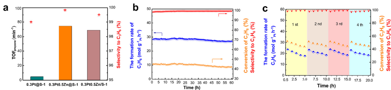
Fig. 19 (a) The TOF of Pt-based catalysts at 450\text{ }^{\circ}\text{C} ; (b) stability testing over 0.3Pt0.5Zn@S-1 at 550\text{ }^{\circ}\text{C} for 60 h; (c) recyclability of 0.3Pt0.5Zn@S-1 in the PDH reaction at 600\text{ }^{\circ}\text{C} (reaction conditions: 200 mg catalysts, atmospheric pressure, \text{WHSV}_{\text{propane}} = 6.5\text{ h}^{-1} , and \text{C}_3\text{H}_8:\text{N}_2 = 11:19 with flow rate 30\text{ mL min}^{-1} ). 136 Reprinted with permission from Elsevier Inc., copyright 2020.
