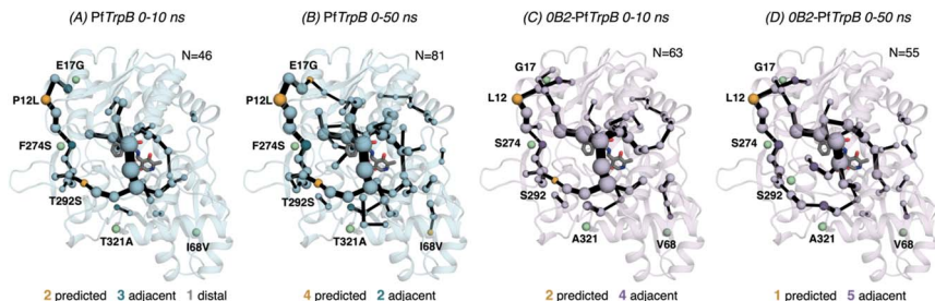
Fig. 5 Evolution of the SPMs along the MD time. The number of identified conformationally relevant positions (N) is increased from 46 to 81 in the case of (A and B) PflTrpB , and slightly decreased from 63 to 55 in (C and D) OB2-PflTrpB . The size of spheres and the thickness of edges in the SPM plots are weighted according to their importance for the conformational dynamics of the enzyme: those pairs of residues that have a higher contribution to the conformational dynamics are represented with a thicker edge and larger sphere. All SPM graphs have been generated using the default settings: a threshold of 6.0 Å for the distance matrix, and a 0.3 for the significance threshold.
