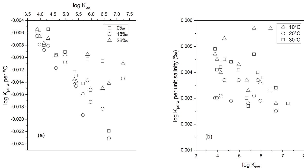
Fig. 3 Temperature effects (determined by the change in log K_{PE-W} per °C) versus log K_{OW} (a) and the salinity effects (determined by the change in log K_{PE-W} per unit salinity (‰)) versus log K_{OW} (b). The regression equation for temperature effects in the absence of salt ( i.e. , 0‰) = -0.0041 \log K_{OW} + 0.010 ( r^2 = 0.69 ).
