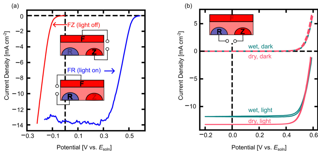
Fig. 4 Photovoltaic, electrochemical, and electrical characterization of the three-operating modes of 3T n-labeled BC Si in both the light and in the dark. (a) Illuminated FR mode CV and dark FZ mode CV vs. E_{\text{soln}} immersed in MV^{2+/+} solution. (b) Illuminated and dark RZ mode CVs for an electrode measured in air (dry) and in MV^{2+/+} electrolyte (wet, E_{\text{soln}} = -0.5 V vs. Ag/AgCl). All illuminated data measured under simulated AM1.5G spectra. Insets show schematics of the contacts used for FR, FZ and RZ measurements.
