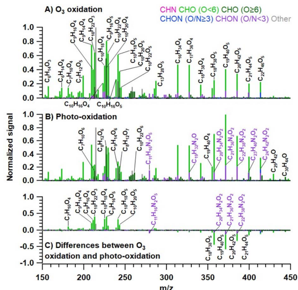
Fig. 2 High-resolution mass spectra of the observed species produced under (A) ozone oxidation reaction, (B) photo-oxidation oxidation reaction, and (C) comparison of both spectra calculated by graph (A) minus graph (B). The signal is normalized to the maxima of the highest peaks observed. Due to space constraints, only the species with the highest relative signal intensity are labelled in this figure. The labelled species in the figure have omitted the \text{Na}^+ ion.
