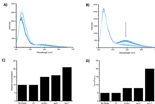
Fig. 30 Emission spectra of 87 (20 \mu\text{M} ) in DMSO (1% \text{H}_2\text{O} ) upon addition of \text{TBA}_2\text{SO}_4 (0 to 60 equiv.) ( \lambda_{\text{ex}} = 280 \text{ nm} ) at 298 K (A). Emission spectra 88 (20 \mu\text{M} ) in DMSO/1% \text{H}_2\text{O} upon addition of \text{TBA}_2\text{SO}_4 (0 to 80 equiv.) ( \lambda_{\text{ex}} = 280 \text{ nm} ) at 298 K (B). The ratios of I_{325}/I_{490} for 87 (C) and 88 (D) in DMSO/1% \text{H}_2\text{O} at 298 K in the presence of anion (10 equiv.). Adapted with permission from ref. 82. Copyright RSC 2023.
