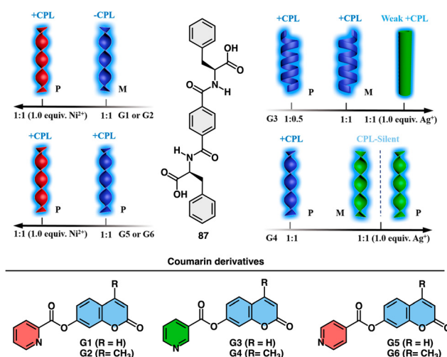
Fig. 34 Schematic representation of the co-assembly of chiral LPF ( 87 ) and achiral fluorescent coumarin derivatives ( G1–G6 ) and their response to metal ions ( \text{Ni}^{2+} and \text{Ag}^+ ). Reproduced from ref. 215 with permission from the American Chemical Society, copyright 2019.
