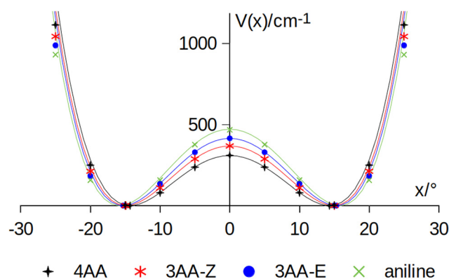
Fig. 8 Amine inversion potential energy function. Points are calculated at the MP2/aug-cc-pVTZ level using a sample step of 5°. Lines correspond to the double minimum function described in eqn (3) using the theoretical barriers and pyramidalization angles ( x ) listed in Table 8.
