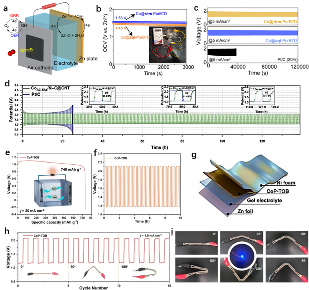
Fig. 9 (a) Schematic illustration of the Zn-air battery (ZAB). (b) The open circuit curves of the ZAB using \text{Co}@sql\text{-PorBTD} and \text{Co}@rhm\text{-PorBTD} . (c) The discharge/charge cycling measurement of ZAB using \text{Co}@sql\text{-PorBTD} , \text{Co}@rhm\text{-PorBTD} , and 20 wt% Pt/C. (Reproduced with permission of ref. 73, Copyright 2023 American Chemical Society.) (d) Charge-discharge cycling performance of ZAB using \text{Co}_{AC-SAS}/\text{N-C}@CNT and Pt/C. (Reproduced with permission of ref. 77, Copyright 2023, Beijing Institute of Technology Press.) (e) Discharge capacity of a ZAB using CoP-TOB. (f) Galvanostatic discharge-charge cycling measurement of ZAB using CoP-TOB at 2 mA cm -2 . (g) Schematic diagram of a flexible solid-state ZAB. (h) Discharge-charge polarization plots under different bent conditions. (i) Photographs of a LED lit by the ZAB under bent conditions. (Reproduced with permission of ref. 53, Copyright 2023, Wiley VCH.)
