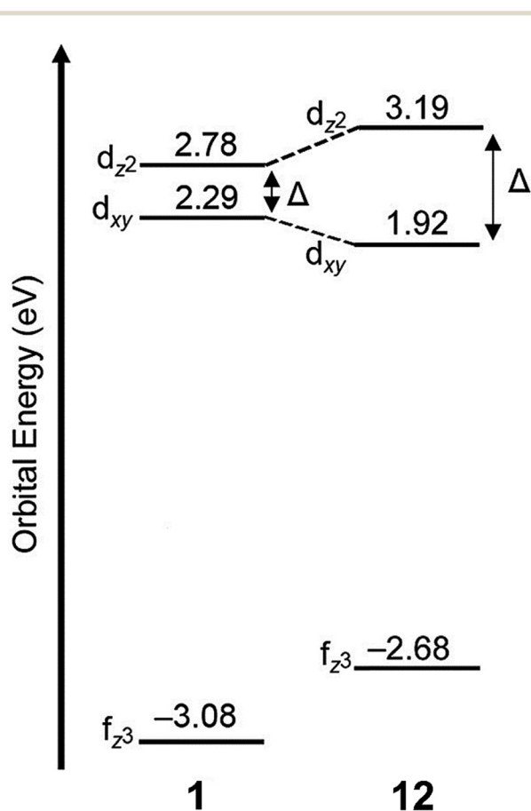
Fig. 8 Calculated d-orbital splitting of \text{Eu}^{\text{II}} 1 and \text{Eu}^{\text{II}} 12. Adapted from Corbin et al. , 81 copyright 2018, with permission from Elsevier.
