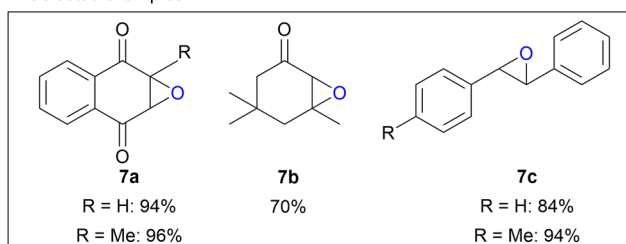
Scheme 3 Epoxidation of unsaturated \alpha,\beta -enones with 1 .
