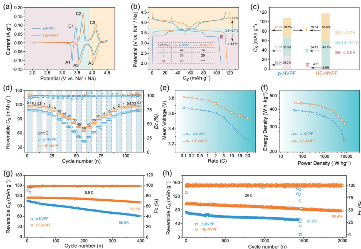
Fig. 15 Electrochemical properties of HE-NVPF and p-NVPF tested in coin-type half-cells. (a) CV patterns at a scan rate of 0.1 mV s -1 . (b) GCD curves at 0.1 C in the potential windows of 2.0–4.3 V versus Na + /Na. (c) Discharge C s values and capacity contribution rates of discharge voltage intervals calculated from the discharge curves in (b). (d) Rate capability. (e) V m variations calculated based on the discharge curves along with rates. (f) Ragone plots. (g) and (h) Cycling performance at 0.5 C and 20 C. Copyright permission from Wiley, used from ref. 42.
