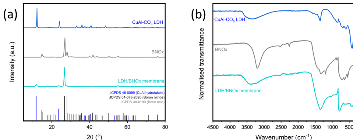
Fig. 1 (a) pXRD patterns and (b) FT-IR spectra of CuAl-CO 3 LDHs (blue), BNOx (grey) and LDH/BNOx nanocomposite (turquoise). pXRD reference patterns are provided for CuAl hydroxalite, boron nitride and boric acid.
