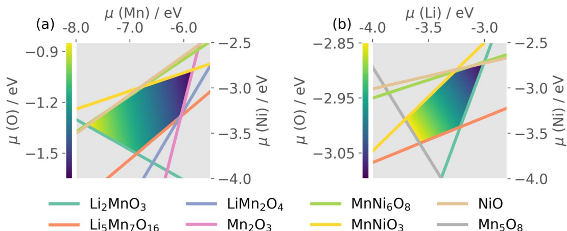
Fig. 3 The chemical potential space of P_{43/32} \text{LiMn}_{1.5}\text{Ni}_{0.5}\text{O}_4 , (a) where chemical potential of Li was set to an average value of -3.35 eV; (b) where chemical potential of Mn was set to an average value of -6.42 eV. Yellow/dark-blue colour shadings represent p/n-type conditions.
