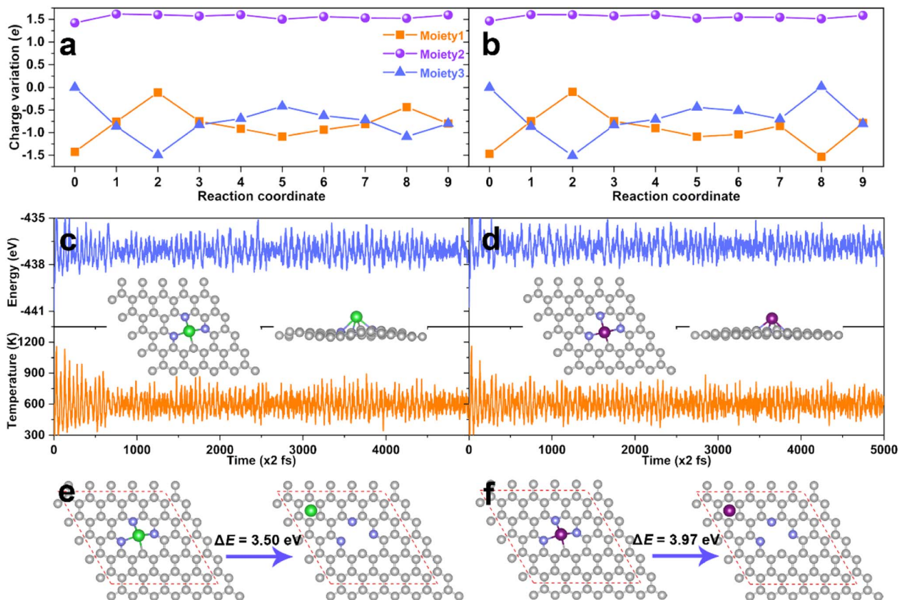
Fig. 8 The charge variation during the e\text{NO}_3\text{RR} process on DV- \text{BaN}_3\text{C} (a) and DV- \text{SrN}_3\text{C} (b). Energy and temperature evolution during the AIMD simulation for DV- \text{BaN}_3\text{C} (c) and DV- \text{SrN}_3\text{C} (d). Insets are the top and side views of the snapshots after 10 ps. The most stable configuration and second stable one with the Ba (e) and Sr (f) near the hollow sites, where \Delta E is their energy difference.
