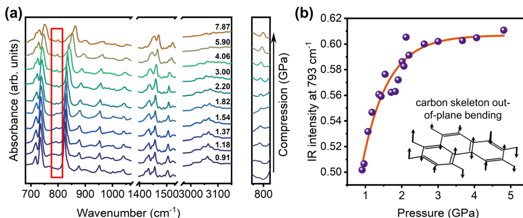
Fig. 2 (a) In situ IR spectra of the phenanthrene crystal upon compression. (b) The pressure-dependent IR absorption intensities around 793 \text{cm}^{-1} and the schematic diagram of the corresponding vibrational mode. The relevant vibrations are marked in the diagrams (a).
