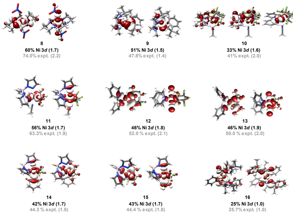
Fig. 7 Frontier unoccupied/singly occupied MOs of formally \text{Ni}^{\text{III}} and \text{Ni}^{\text{IV}} species. Calculated (black) and experimental (grey) averaged % Ni 3d contributions are printed below the orbitals. Corresponding 3d-vacancies are given in parentheses. Orbitals were calculated at the B3LYP/CP(PPP)/ZORA-def2-TZVP(-f) level and plotted at an isovalue of 0.03 au.
