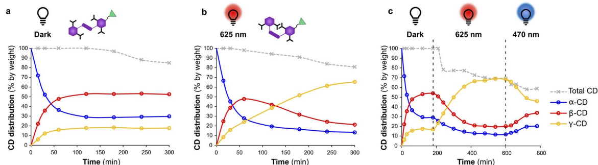
Fig. 5 Distribution of \alpha -, \beta -, and \gamma -CD as function of time for enzymatic reactions starting from \alpha -CD ( 10 \text{ mg mL}^{-1} ) with CGTase ( 65 \text{ } \mu\text{L mL}^{-1} reaction mixture) in sodium phosphate buffer (100 mM, pH 7.5) in the presence of template ipAzo (10 mM). Reaction conditions: (a) in darkness having primarily the trans isomer, (b) under continuous red light irradiation (625 nm) promoting trans to cis isomerisation and (c) starting in darkness, then under irradiation with red light and finally under irradiation with blue light (470 nm) to promote cis to trans isomerisation.
