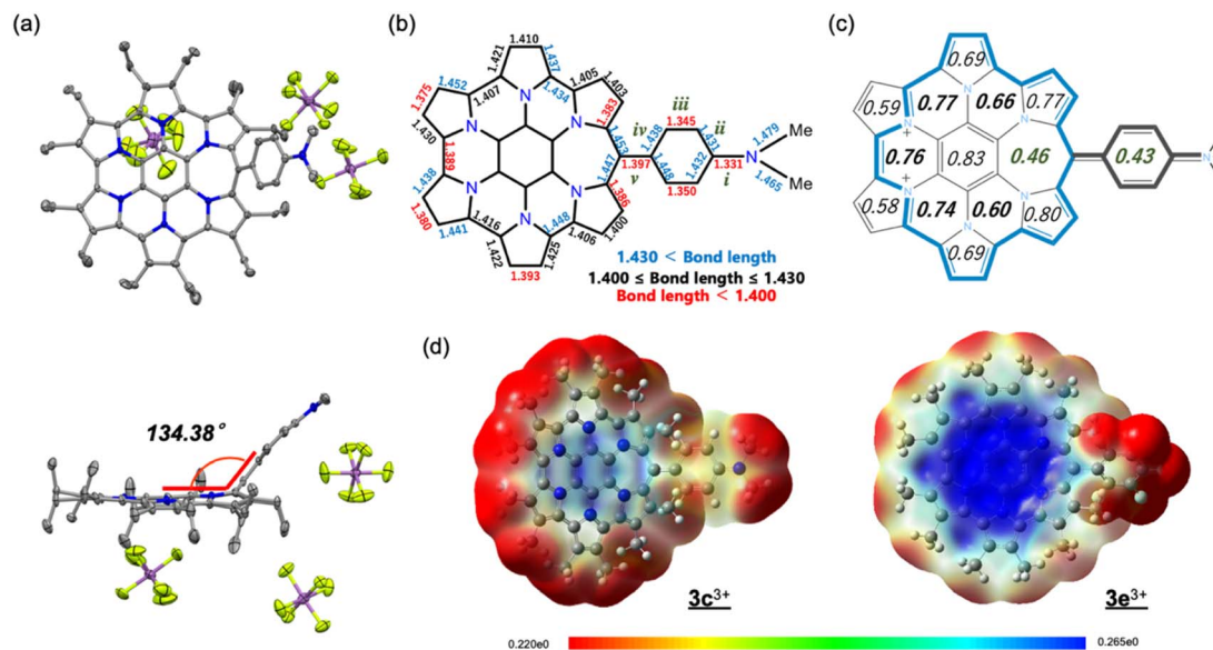
Fig. 7 (a) Crystal structures (top and side views) of 3c^{3+}[\text{SbF}_6^-]_3 . Thermal ellipsoids are scaled to 50% probability. Solvent molecules and disordered atoms are omitted for clarity. (b) Selected bond lengths (Å) and (c) HOMA values of the crystal structure of 3c^{3+}[\text{SbF}_6^-]_3 . (d) ESP plots of 3c^{3+} and 3e^{3+} calculated at the B3LYP/6-31G(d) level of theory, in which the Et groups are replaced with Me groups to simplify the calculations.
