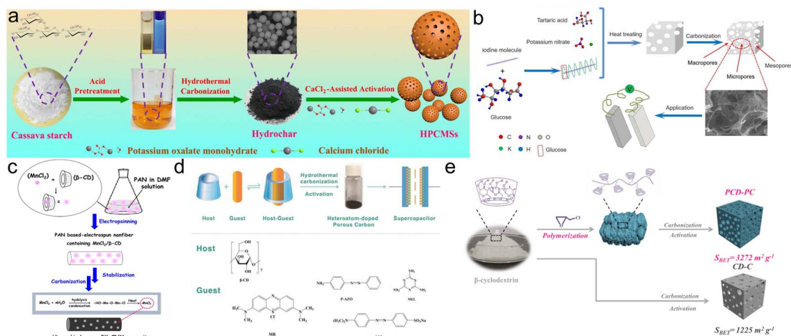
Fig. 6 (a) Illustration for the synthesis of HPCMSs; 64 (b) scheme for the preparation of I-PCs-X; 66 (c) diagram for the construction of PMnCD(β); 67 (d) schematic for the preparation mechanism of porous CMs; 68 (e) mechanism diagram for the synthesis of the PCD-PC. 69
