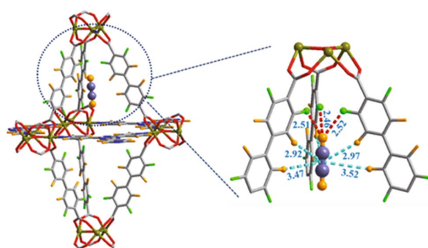
Fig. 17 Preferential C 2 H 2 adsorption site calculated from GCMC simulation for JXNU-12(F). Element key: Ni (dark yellow), C (gray), F (bright green), O (red) and H (bright orange). Reproduced from ref. 62 with permission from Elsevier, copyright 2022.
