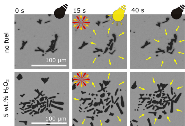
Fig. 4 Collective swarming behavior of microrobots as a function of UV irradiation. Comparison of fueled and non-fueled microrobots.
