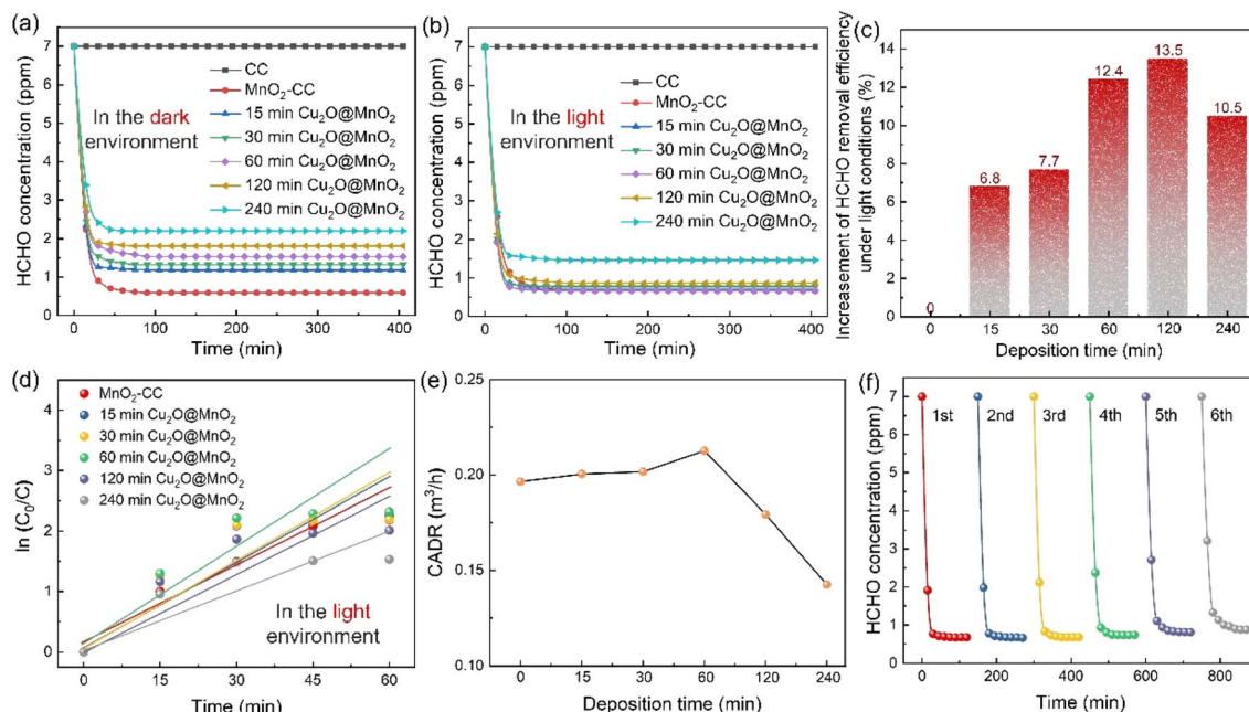
Fig. 3 HCHO concentration changes with time under the action of CC, \text{MnO}_2 -CC and \text{Cu}_2\text{O}@\text{MnO}_2 (a) in the dark state and (b) in the light environment. (c) Efficiency increase, (d) first-order reaction fitting and (e) the available clean air volume (CADR) calculation values for HCHO static removal efficiency by different catalysts. (f) Thermal regeneration tests of "60 min \text{Cu}_2\text{O}@\text{MnO}_2 " over 6 cycles.
