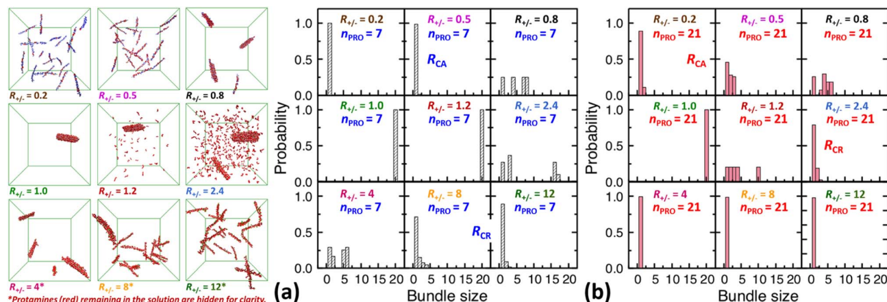
Fig. 3 Final snapshots taken after 120 ns as well as DNA bundle size ( N_{\text{DNA}} = 1-20 ) distributions averaged over the last 20 ns of unbiased MD simulations started from homogeneous DNA solutions mixed with (a) 7-bead or (b) 21-bead protamine at R_{+/-} of 0.2, 0.5, 0.8, 1, 1.2, 2.4, 4, 8, and 12. \text{Na}^+ (blue) and \text{Cl}^- (green) as well as some 7-bead protamine (red) remaining in the solution, i.e. , not bound to DNA (grey), are hidden for clarity. The R_{\text{CA}} and R_{\text{CR}} denote the onset R_{+/-} of DNA aggregation and redissolution, respectively, upon adding protamine to the solution. The average over 20 independent runs performed at R_{+/-} of 0.5 and 2.4 are shown in Fig. S4-2, Section S4, ESI†
