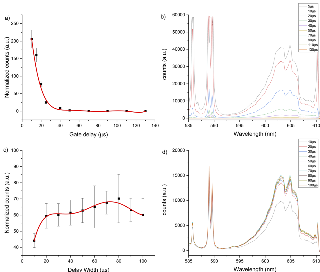
Fig. 4 LIBS signal optimization under argon flow of 1 \text{ L min}^{-1} for 600 nm window using a 2500 \mu\text{g g}^{-1} hydroxyapatite standard. (a) Gate delay optimization maintaining constant gate width at 50 \mu\text{s} , (b) LIBS spectrum for each gate delay change, (c) gate width optimization maintaining constant gate delay at 20 \mu\text{s} , (d) LIBS spectrum for each gate width change.
