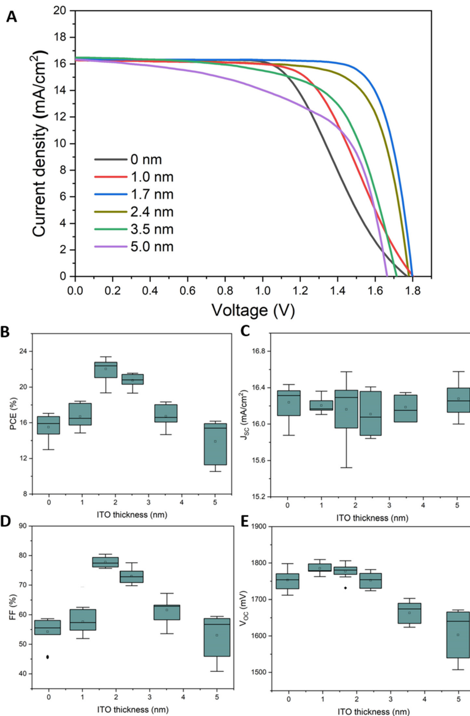
Fig. 2 Effect of the ITO inter-layer thickness on the performance of 1 cm 2 tandem test solar cells (before the application of front anti-reflection control). (A) J - V curve of the champion testing tandem devices with different ITO interlayer thicknesses. Distribution of (B) PCE, (C) short-circuit current density ( J_{sc} ), (D) fill factor (FF), and (E) open circuit voltage ( V_{oc} ) based on 10 devices for each condition. The highest value is the maximum value. The highest bar is the 75 th percentile value. The middle bar is the median value. The square mark is for the average. The lowest bar is the 25 th percentile value. The lowest value is the minimum.
