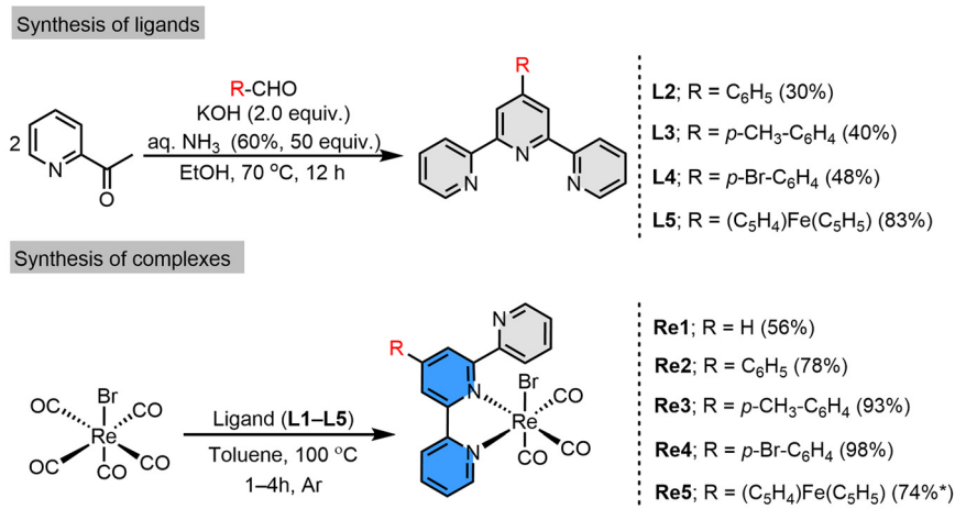
Scheme 1 Synthesis of terpyridine ligands (L2–5) and fac - \text{Re}(\text{i})(\text{L})(\text{CO})_3\text{Br} complexes (Re1–5), where L = L1–5. *Re5 contains toluene (~0.5 molecules, calculated from ^1\text{H} NMR) as a solvent of crystallisation.
