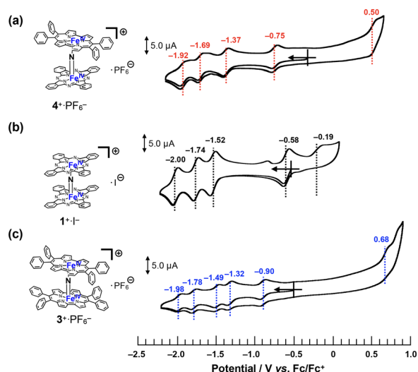
Fig. 5 Comparison of cyclic voltammograms of (a) 4^+\cdot\text{PF}_6^- , (b) 1^+\cdot\text{I}^- , and (c) 3^+\cdot\text{PF}_6^- in a pyridine solution containing 100 mM of n\text{Bu}_4\text{N}^+\text{PF}_6^- at room temperature. [Substrate] = 200 \mu\text{M} , [scan rate] = 100 \text{mV s}^{-1} .
