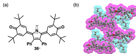
Fig. 22 (a) Deprotonated pyrrole-bridged quinone 36^- and (b) single-crystal X-ray structure of \text{TBA}^+ \cdot 36^- (redrawn from a cif file: 2076443).
