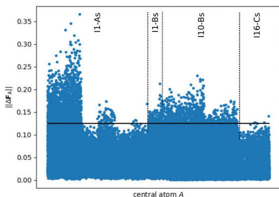
Fig. 7 Norm of the DFT force errors \|\Delta F_A\| (in \text{eV \AA}^{-1} ), i.e. , the absolute difference between the force vectors in the periodic bulk structure and in the small fragments ( R_{\text{frag}} = 4.359 \text{ \AA} , cf. Fig. 3), for all central atoms with a complete environment within R_c . The criterion for converged forces \|\Delta F^{\text{max}}\| \leq 0.125 \text{ eV \AA}^{-1} ( conf. ref. 48) is highlighted by the black line showing that a significant part of the atomic forces in the fragments is substantially different from the periodic bulk system.
