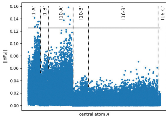
Fig. 6 Norm of the DFT force errors \|\Delta F_A\| (in \text{eV \AA}^{-1} ), i.e. , the absolute difference between the force vectors in the periodic bulk structure and in the large fragments ( R_{\text{frag}}^{\text{conv}} = 8.718 \text{ \AA} , cf. Fig. 5), for all central atoms in a bulk-like environment. The target accuracy for converged forces \|\Delta F^{\text{max}}\| = 0.125 \text{ eV \AA}^{-1} ( cf. ref. 48) is highlighted by the black line showing that the vast majority of atomic forces in the fragments is very similar to the periodic bulk system.
