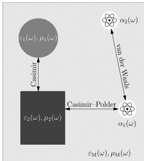
Fig. 13 Schematic illustration of dispersion interactions: Casimir force between two dielectric macroscopic objects with permittivities \varepsilon_i and permeabilities \mu_i , the Casimir-Polder force acting between a polarisable object \alpha_1 and the dielectric body \varepsilon_2 , and the van der Waals force interacting between two polarisable objects \alpha_i .
