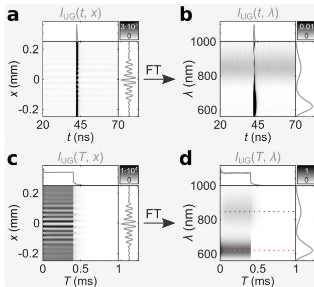
Fig. 2 Ungated bmFSTS data of (DNA)_2[Ag_{18}]^{12+} in an aqueous solution at RT with 520 nm excitation ( I = 3.4 kW cm -2 , f_{Micro} = 13 MHz, f_{Macro} = 1 kHz, T_{on} = 0.4 ms, T_{off} = 0.6 ms). Micro-time domain (a) TRIM and (b) TREM. Macro-time domain TRIM (c) and TREM (d). The blue and red dashed lines in (d) indicate the maxima of the long- and short-lived bands, respectively.
